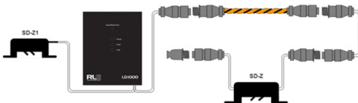
Spot detector example: use the SD-Z and SD-Z1 in conjunction with an RLE SeaHawk leak detection controller.
